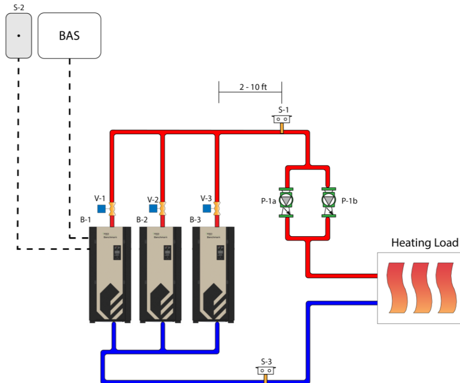
Diagram 4-1a: Space Heating Piping
